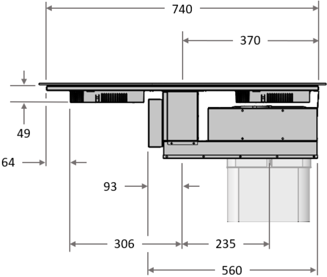
View A
